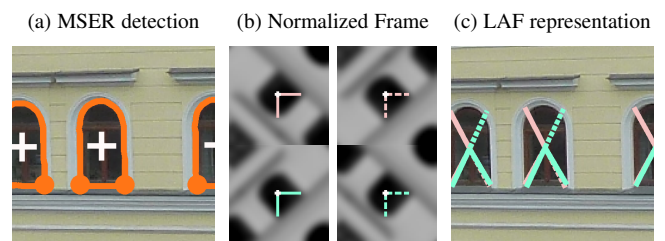
Fig. 8. Repeat Detection, Description, and Representation. (a) Center of gravity (white cross) and curvature extrema (orange circles) of a detected MSER (orange contour [40]). Patches are normalized to a square and oriented to define an affine frame as in [41], (b) Bases are reflected for detecting axial symmetries. The RootSIFT transform embeds the local texture [47], [48]. (c) Affine frames are mapped to the image.
