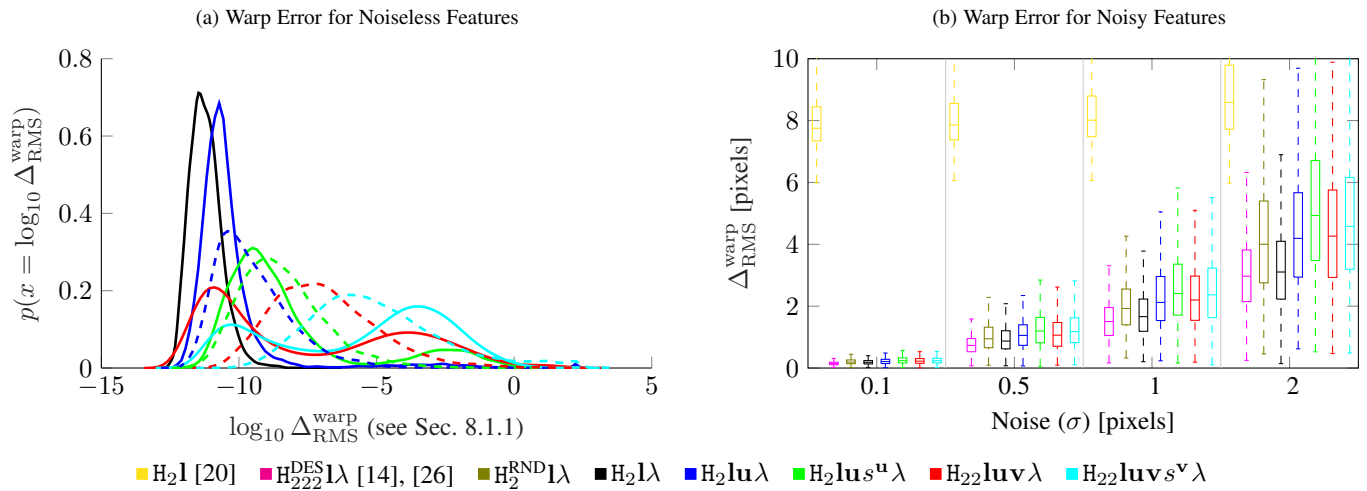
Fig. 9. (a) The \log_{10} RMS warp error \Delta_{\text{RMS}}^{\text{warp}} is reported for noiseless scenes generated as described in Secs. 8.1.1 and 8.1.3. Hidden variable trick solvers are solid; solvers generated without simplified constraints are dashed. The hidden-variable trick increases stability. The EVL H_2\lambda solver is the most stable since it does not require solving a complicated polynomial system of equations. (b) Reports the RMS error \Delta_{\text{RMS}}^{\text{warp}} after 25 iterations of a simple RANSAC for the bench of solvers with increasing levels of white noise added to the affine-covariant region correspondences, where the normalized division model parameter is set to -4, which is similar to the distortion of a GoPro Hero 4. Results are for radially-distorted conjugate translations. The proposed solvers demonstrate excellent robustness to noise, and the EVL solver H_2\lambda is competitive with H_{222}^{\text{DES}}\lambda , which requires two more correspondences. The H_2\lambda solver uses best minimal solution selection, which improves its performance compared to H_2^{\text{RND}}\lambda , which randomly selects a solution.
