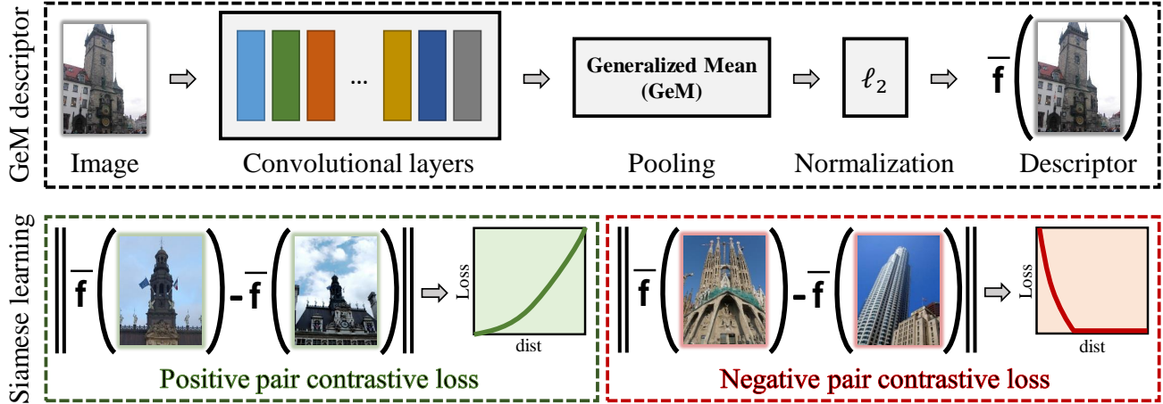
Fig. 1. The architecture of our network with the contrastive loss used at training time. A single vector \bar{f} is extracted to represent an image.
