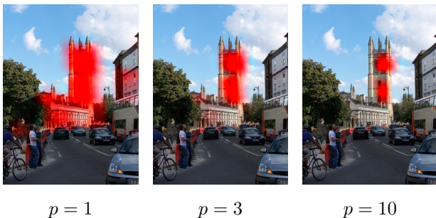
Fig. 4. Visualization of \mathcal{X}_k^p projected on the original image for three different values of p . Case p = 1 corresponds to SPoC, and larger p corresponds to GeM before the summation of (3). Examples shown use the off-the-shelf VGG.
