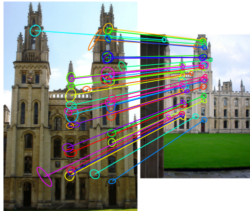
Figure 1. Fast spatial matching [26] finds a linear geometric transformation between two views of an object based on a local feature representation. This is used for spatial verification in large-scale image retrieval. Inlier correspondences shown, colored by visual word. What is the underlying representation? 1
