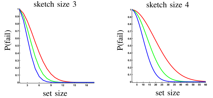
Fig. 4. Probability of failure to generate a seed in a set of images depicting the same object using min-Hash with 512 sketches of size 3 (left) and 4 (right); note the different scales on the horizontal axes. The three curves show the dependence for different ‘average’ similarity equal to 7% (lowest curve), 6% (middle) and 5% (highest).
