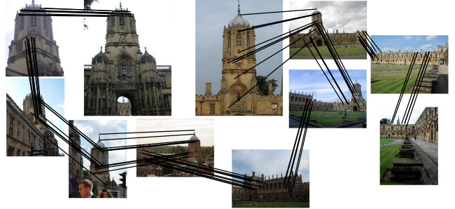
Fig. 1. Visualization of a part of a cluster of spatially related images automatically discovered from a database of 100K images. Overall, there are 113 images in the cluster, all correctly assigned. A sample of geometrically verified correspondences is depicted as links between images. Note that the images show the tower from opposite sides.
