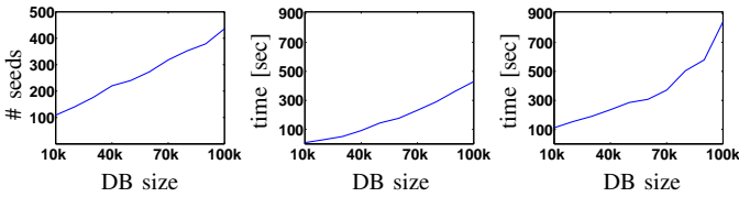
Fig. 6. The number of generated seeds (left), elapsed time of the seed generation (middle), and elapsed time of the cluster completion (right) as a function of the database size. The values are averaged over 10 executions on the 100k Oxford dataset.
