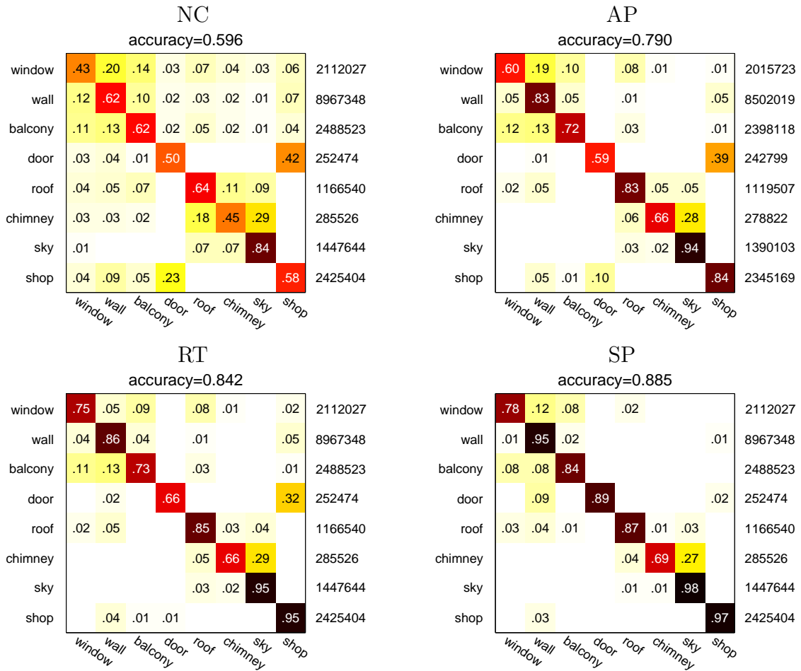
Figure 2: Confusion matrices
