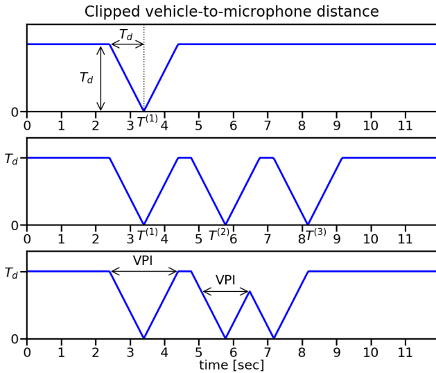
Fig. 4. Clipped vehicle-to-microphone distance (x- and y-axis are in different scale). Top : One vehicle. Middle : Vehicles are apart by at least 2T_d seconds. Bottom : Vehicles are less than 2T_d seconds apart.
