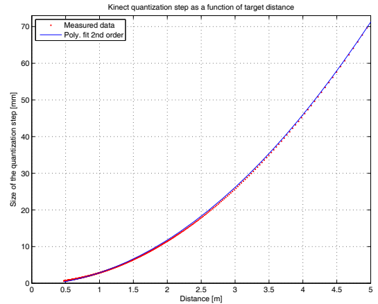
(c) Kinect depth quantization step (0-5 m detail).
