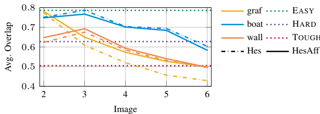
Fig. 4: Average overlap of the Hessian and Hessian-Affine detectors on the viewpoint sequences of [94]. Line color encodes dataset and line style a detector. The selected overlaps of the EASY and HARD variants are visualised with a dotted line.
