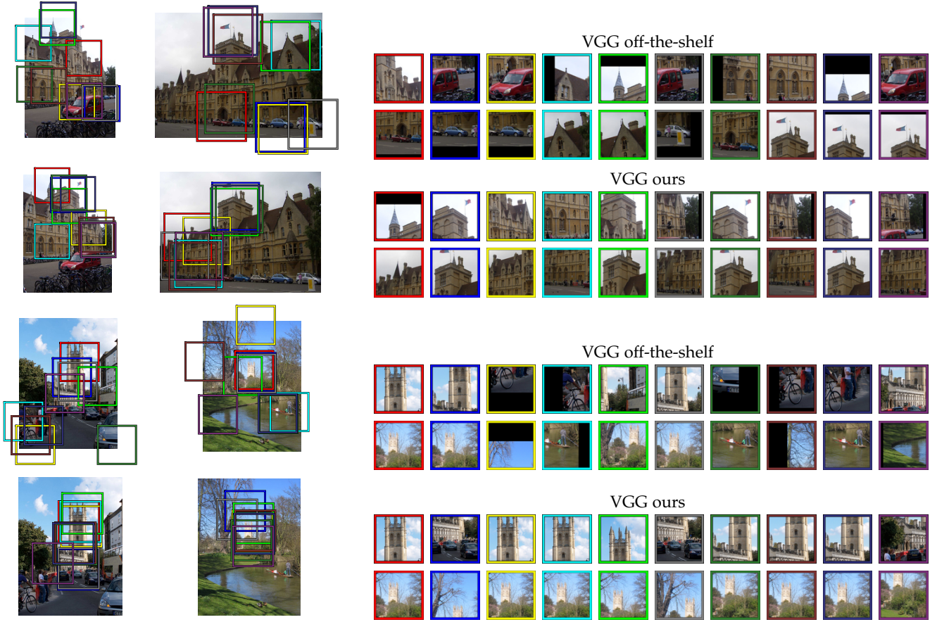
Fig. 2. Visualization of patches corresponding to the MAC vector components that have the highest contribution to the pairwise image similarity. Examples shown use CNN before (top) and after (bottom) the fine-tuning of VGG. The same color corresponds to the same vector component (feature map) per image pair. The patch size is equal to the receptive field of the last pooling layer.
