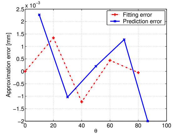
Figure 17: Fitting and prediction error for the proposed model for the FC-E8 lens.
