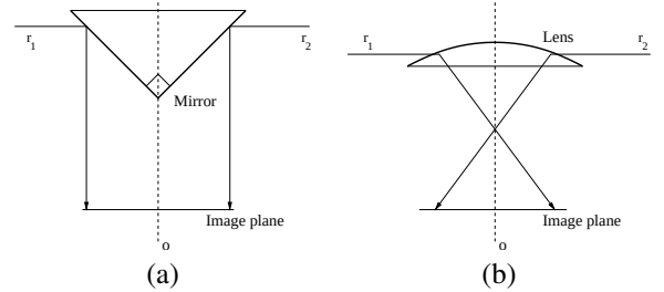
Figure 14: (a) Light rays reflected by the conical mirror are orthographically projected onto a circle. (b) Light rays in one plane are projected by the fish eye lens onto a circle on the sensor.
