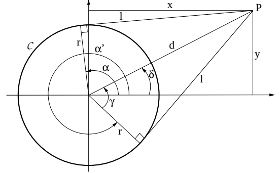
Figure 6: Right symmetric 360 \times 360 mosaic camera geometry - a view in the xy plane.
