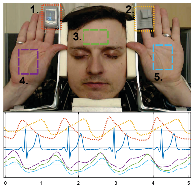
Fig. 1. PPG data acquisition. Top: experimental setup. Bottom: 5 seconds of reference electrocardiogram – navy blue, distinguishable by the QRS-complex, contact transmittance PPG – measured by oximeters on the left and right index fingers (color-coded like areas 1. and 2.), and non-contact reflectance PPG estimated from the video in areas 3., 4., and 5. (NrPPG). The NrPPG signal is high and low pass filtered, and amplified 500 times. Arbitrary units. The head is stabilized in a custom made frame.
