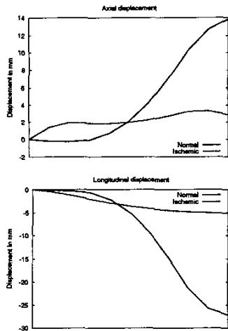
Fig. 3. Axial and longitudinal systolic displacements of a basal septum segment point for a normal volunteer and an ischemic patient with severe hypokinesia.
