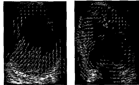
Fig. 2. Displacement field at the mechanical systole for a normal subject ( left ) and an ischemic patient with severe hypokinesia ( right ).
