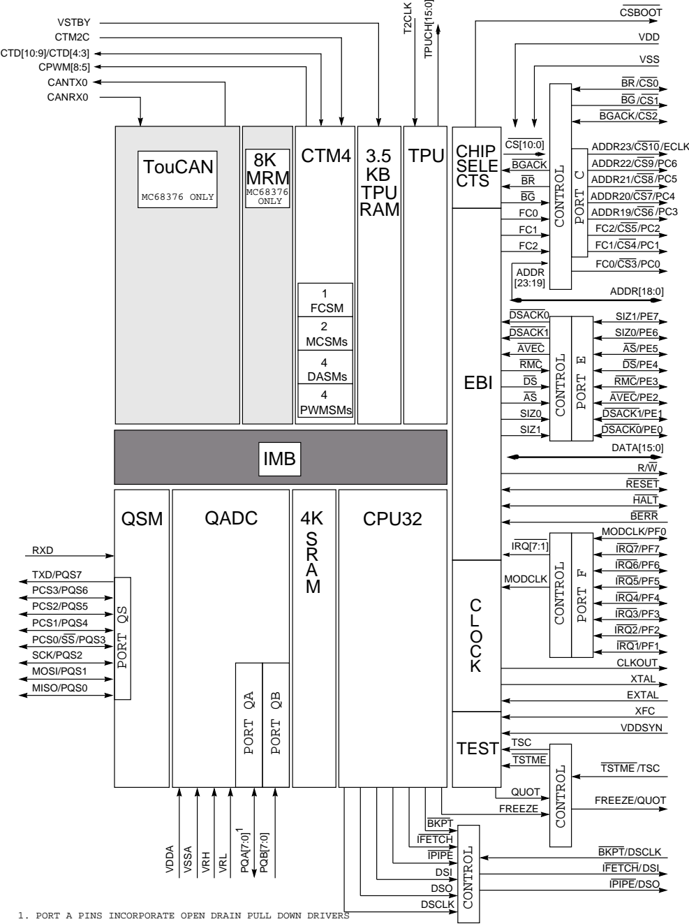
1. PORT A PINS INCORPORATE OPEN DRAIN PULL DOWN DRIVERS
